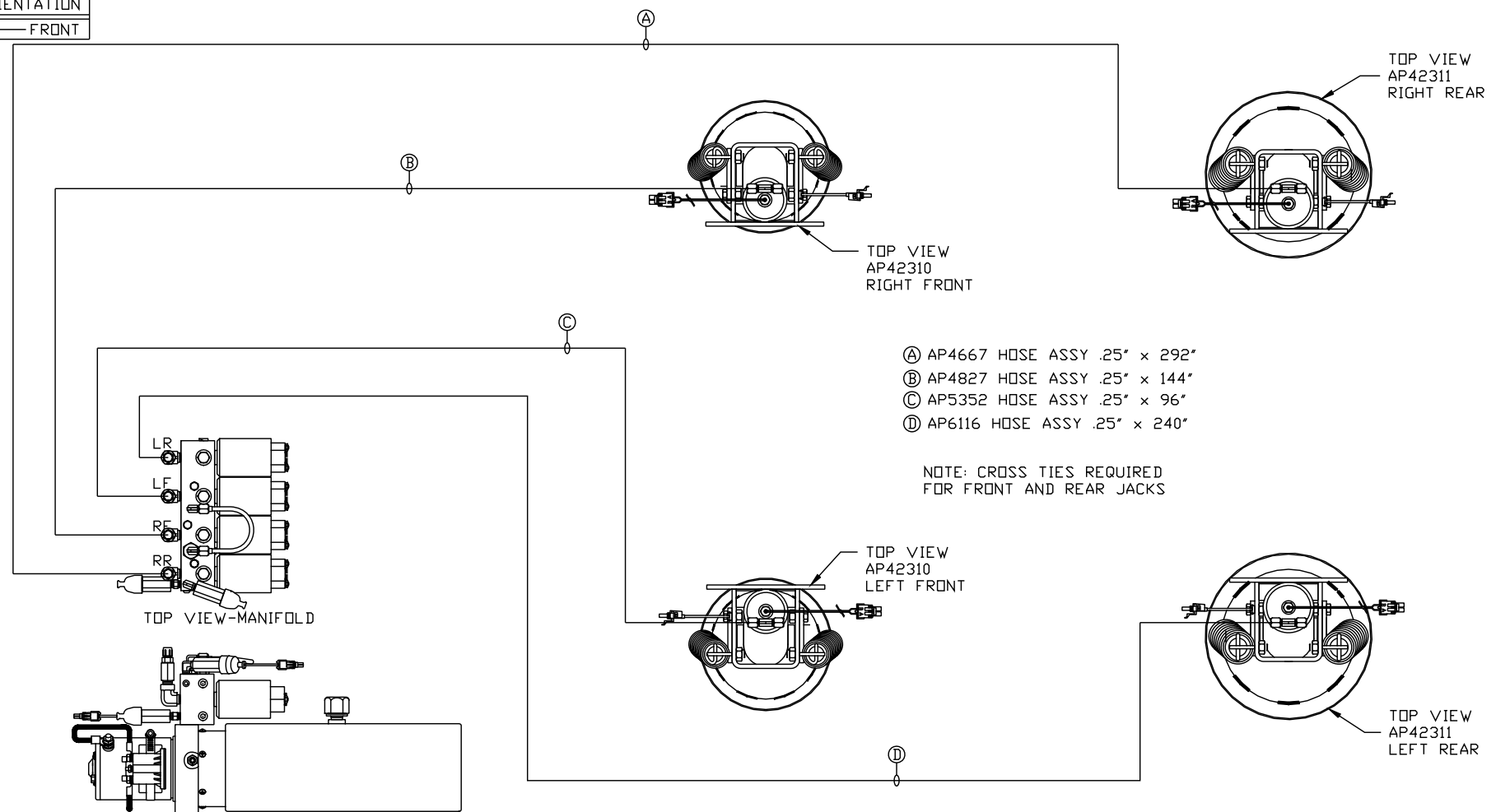
SIDE VIEW PUMP/MANIFOLD-AP38486
