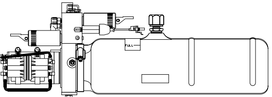
SIDE VIEW PUMP/MANIFOLD-AP46440
