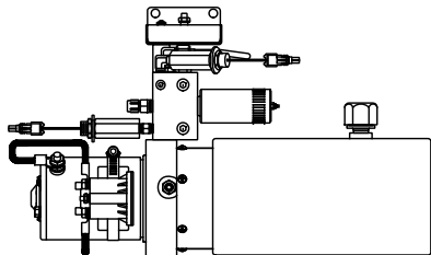
SIDE VIEW PUMP/MANIFOLD-AP47451
