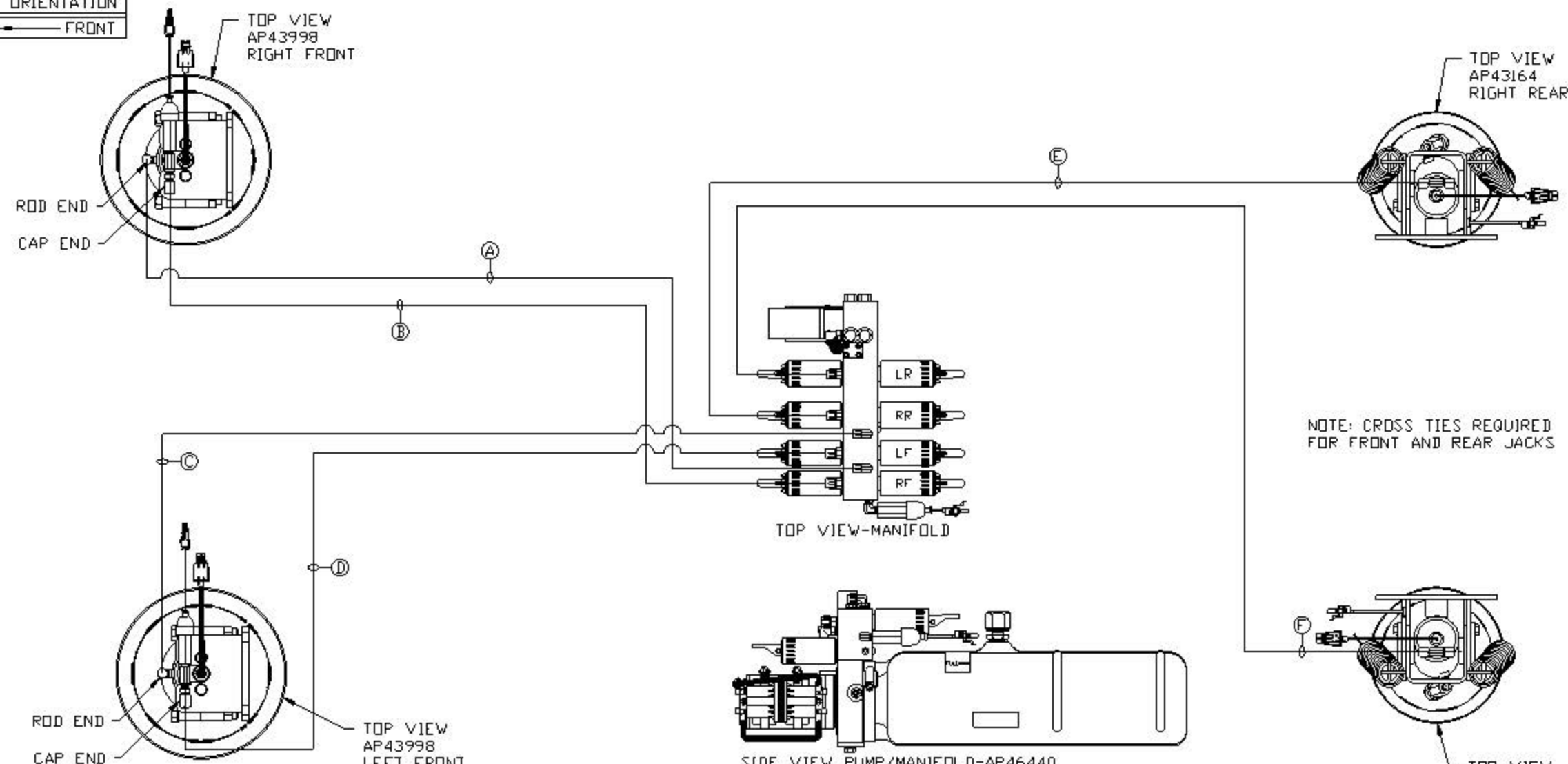
SIDE VIEW PUMP/MANIFOLD-AP46440
