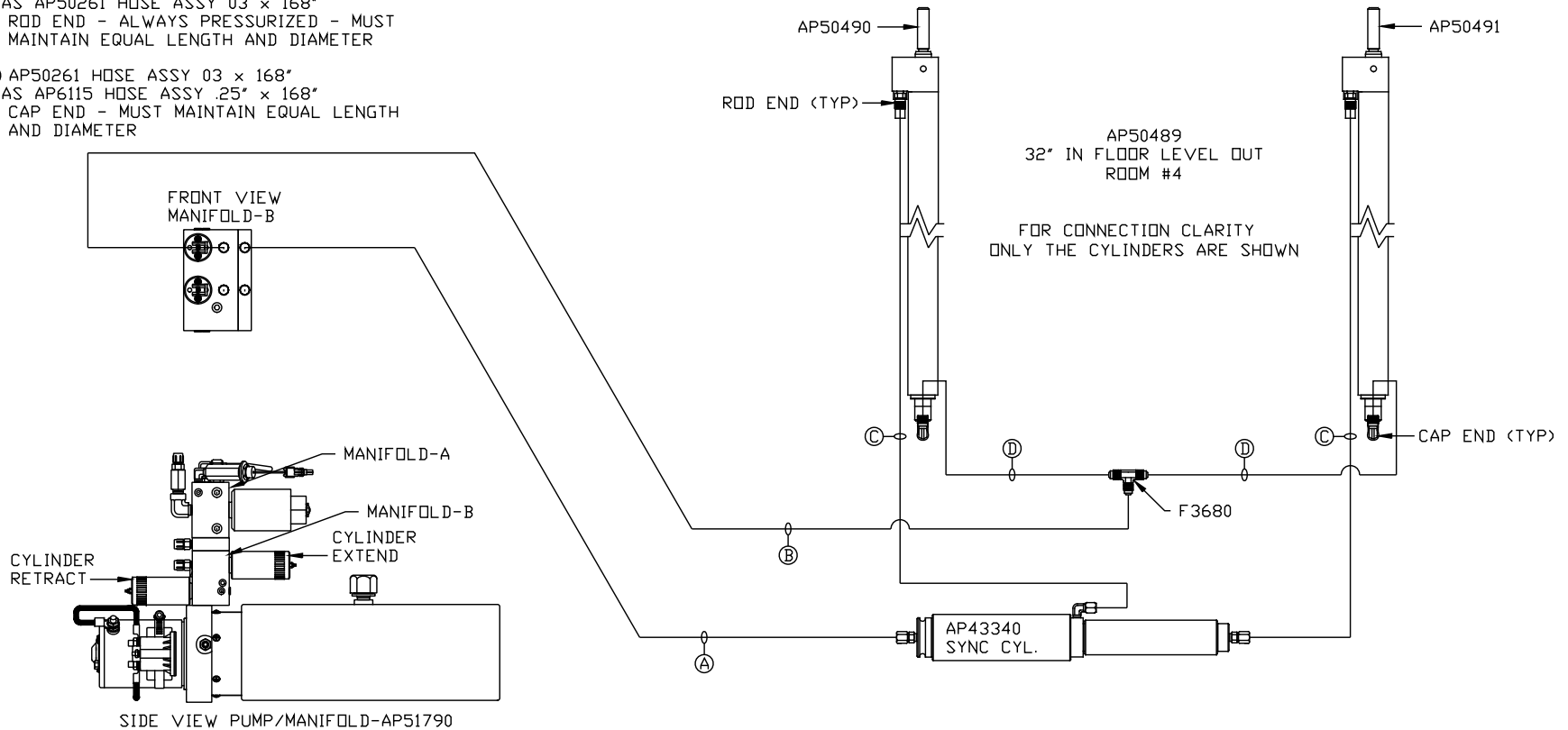
SIDE VIEW PUMP/MANIFOLD-AP51790
