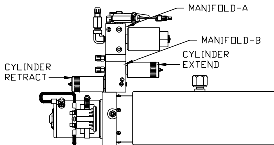
SIDE VIEW PUMP/MANIFOLD-AP51790
