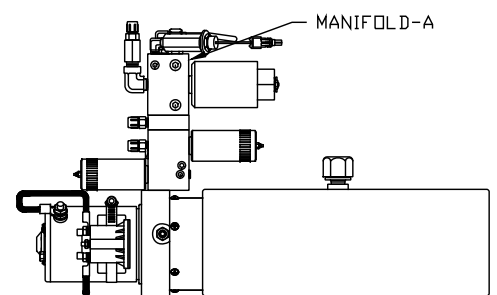
SIDE VIEW PUMP/MANIFOLD-AP51790
