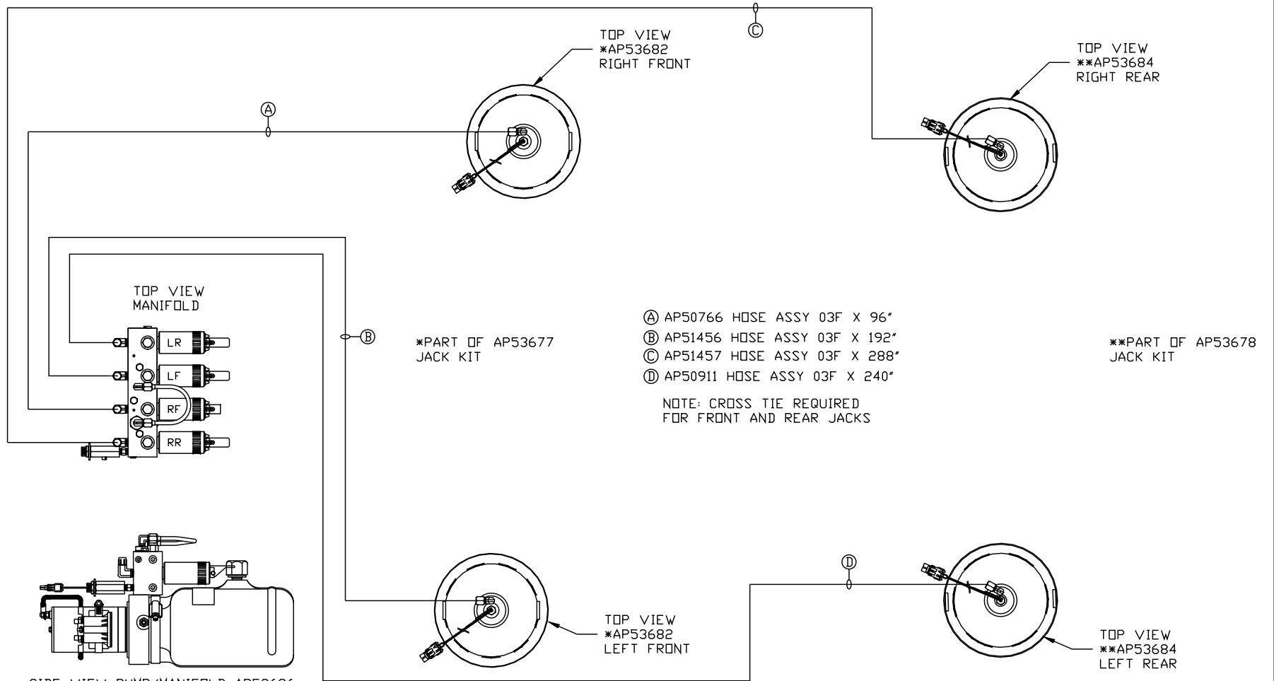
SIDE VIEW PUMP/MANIFOLD-AP53686
