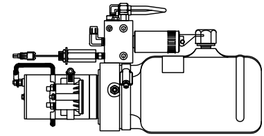
SIDE VIEW PUMP/MANIFOLD-AP53686
