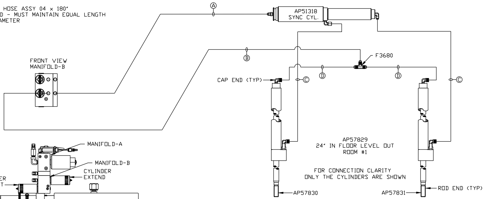
SIDE VIEW PUMP/MANIFOLD-AP54806 LOCATION AND ORIENTATION OF PUMP/MANIFOLD ASSEMBLY WILL DIFFER DEPENDING UPON O.E.M.
