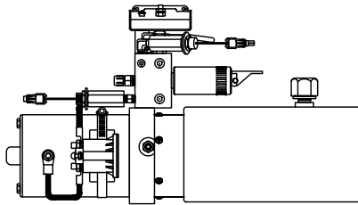
SIDE VIEW PUMP/MANIFOLD-AP58972
