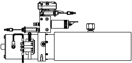
SIDE VIEW PUMP/MANIFOLD-AP58703
