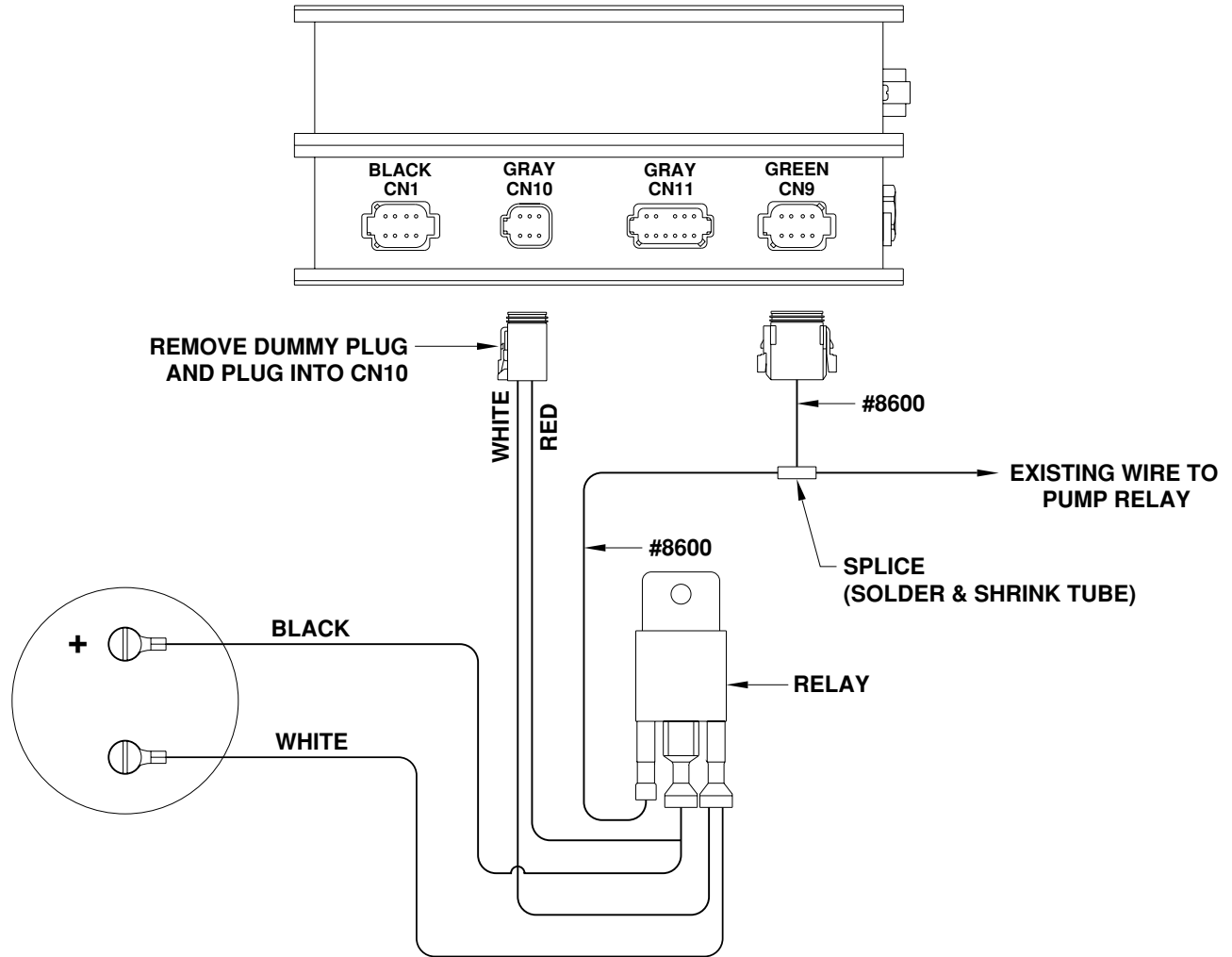
CENTRAL CONTROL MODULE FRONT VIEW
