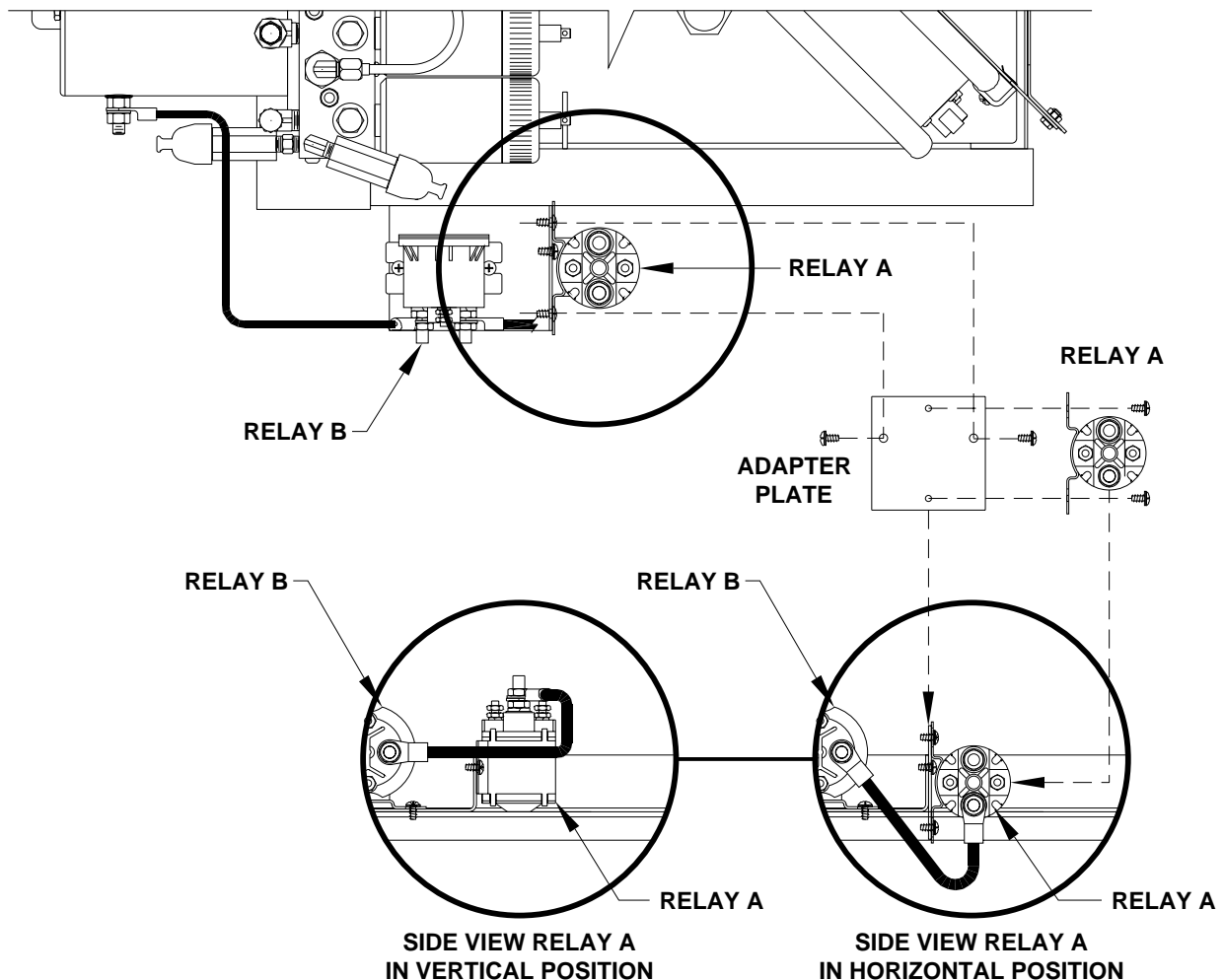
TOP VIEW OF POWER UNIT WITH RELAY A IN THE VERTICAL POSITION
