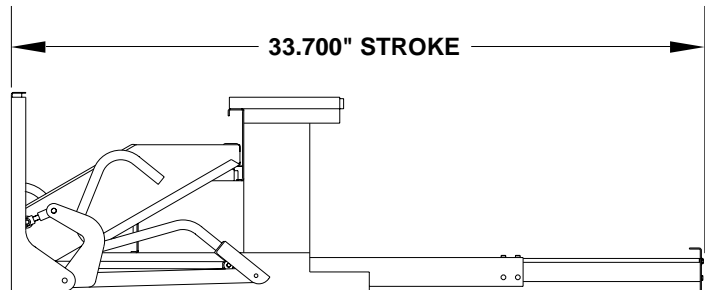
5 STEP - SIDE VIEW - STEP EXTENDED AND UP
