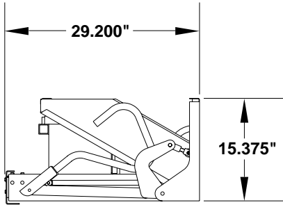
4 STEP - SIDE VIEW - STEP RETRACTED
