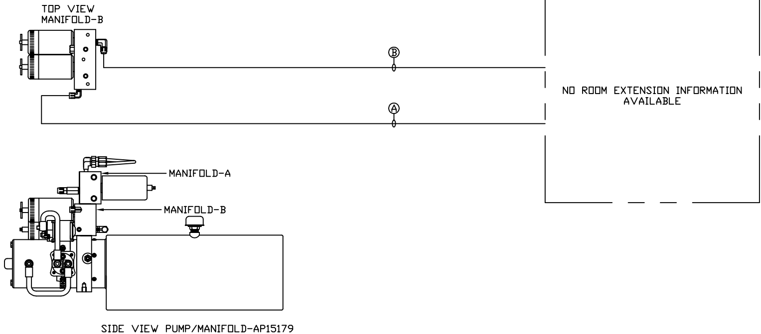
SIDE VIEW PUMP/MANIFOLD-AP15179
