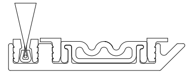
SECTION VIEW: ASSEMBLED RAIL, BRUSH, SEAL, RETAINERS.
