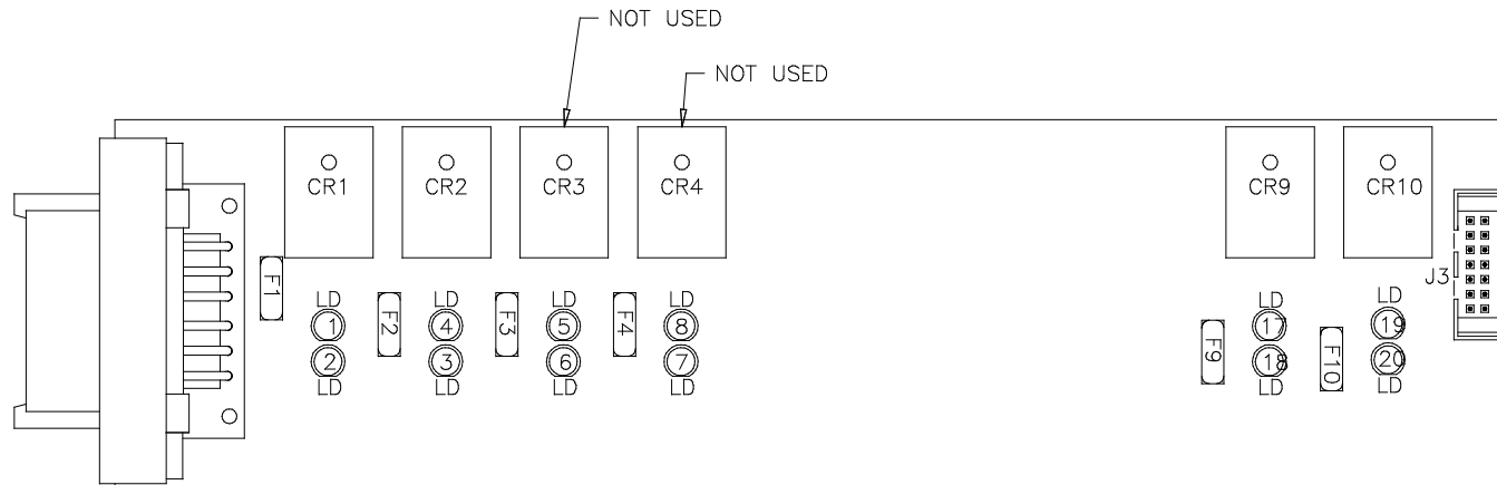
ROOM 1 LED LAYOUT
