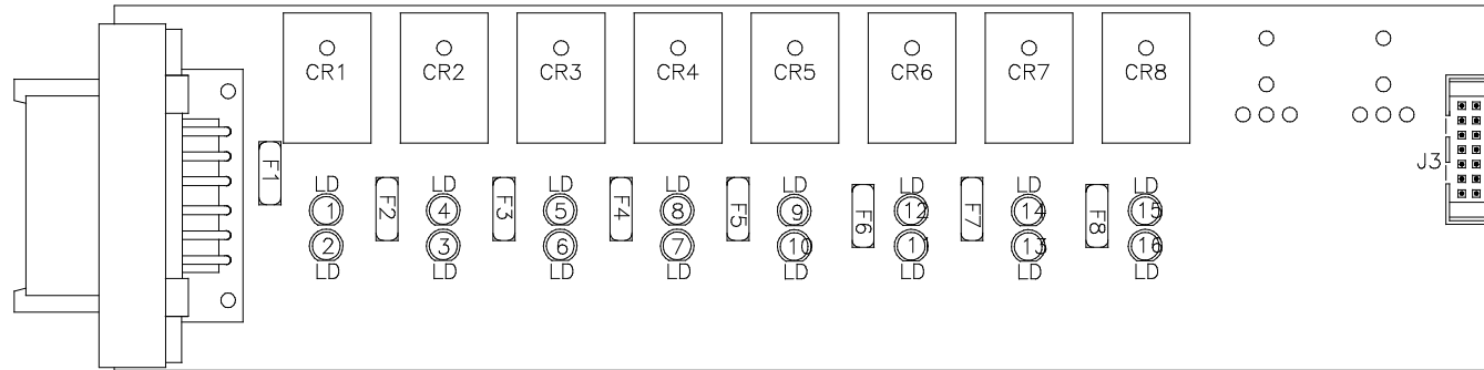
ROOM 1 THROUGH 4 LED LAYOUT
