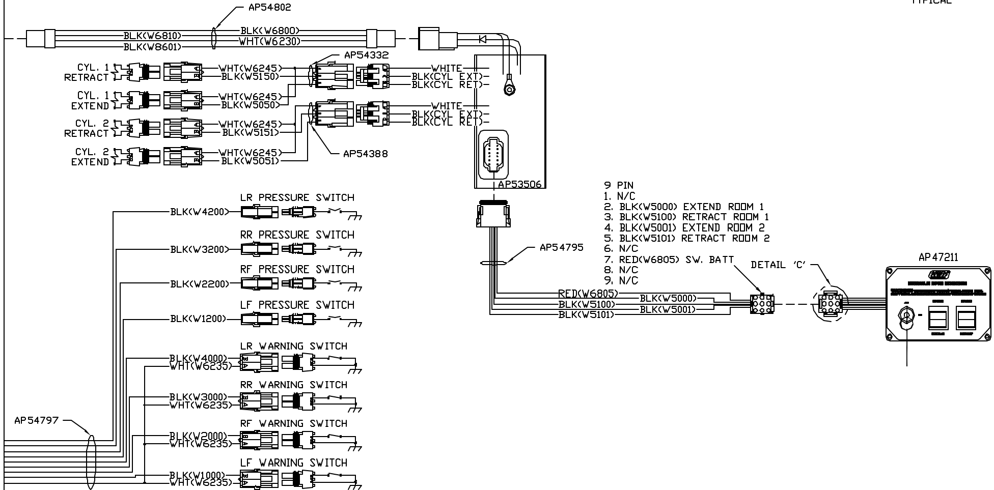
DETAIL 'C' TYPICAL
