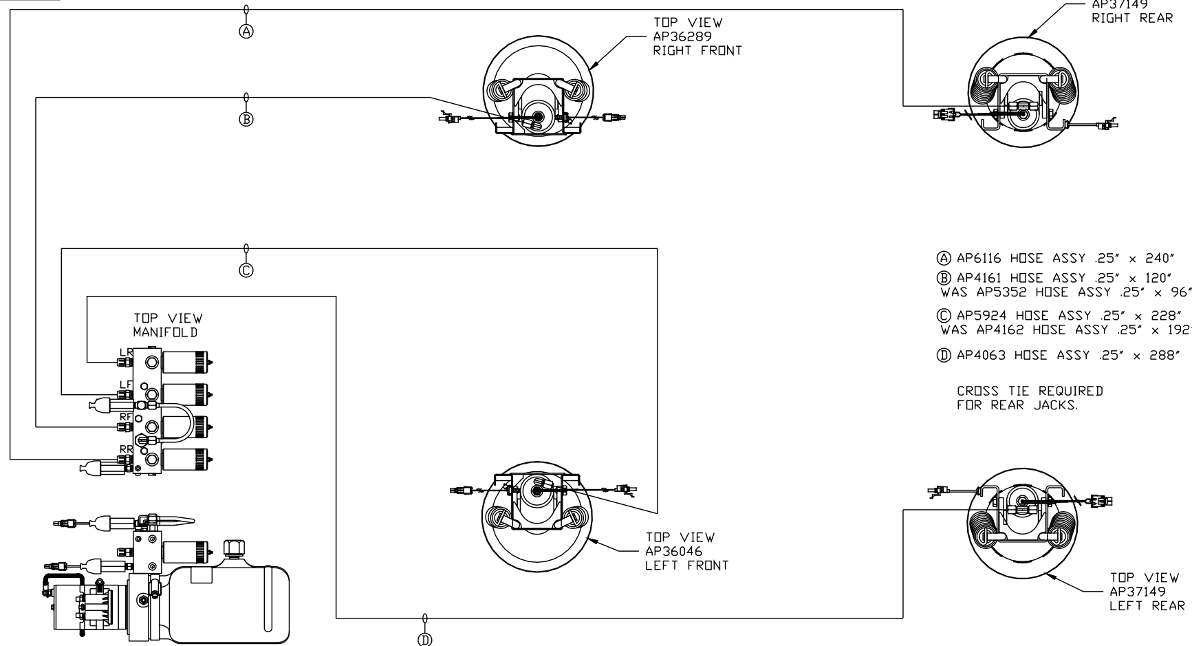
SIDE VIEW PUMP/MANIFOLD-AP40608
