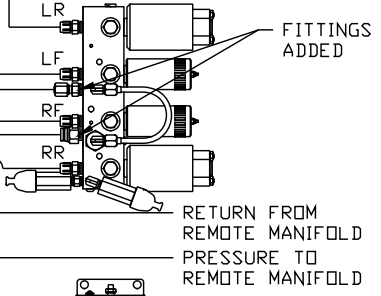
TOP VIEW-MANIFOLD
