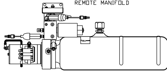
SIDE VIEW PWR/CONTROL-AP46385
