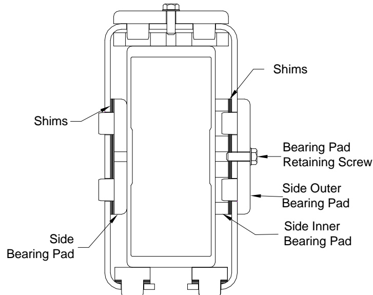
FRONT VIEW OF MECHANISM (FRONT MOUNTING BRACKET OMITTED FOR CLARITY)
