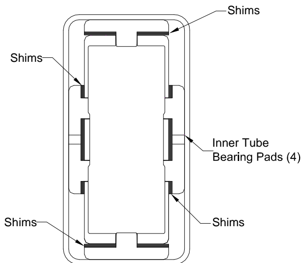
REAR VIEW OF MECHANISM (REAR MOUNTING PLATE OMITTED FOR CLARITY)
