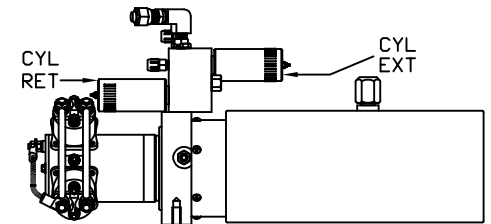
SIDE VIEW OF PUMP/MANIFOLD-AP18161 NOTE: SOME POWER UNITS HAVE LARGE VALVES.
