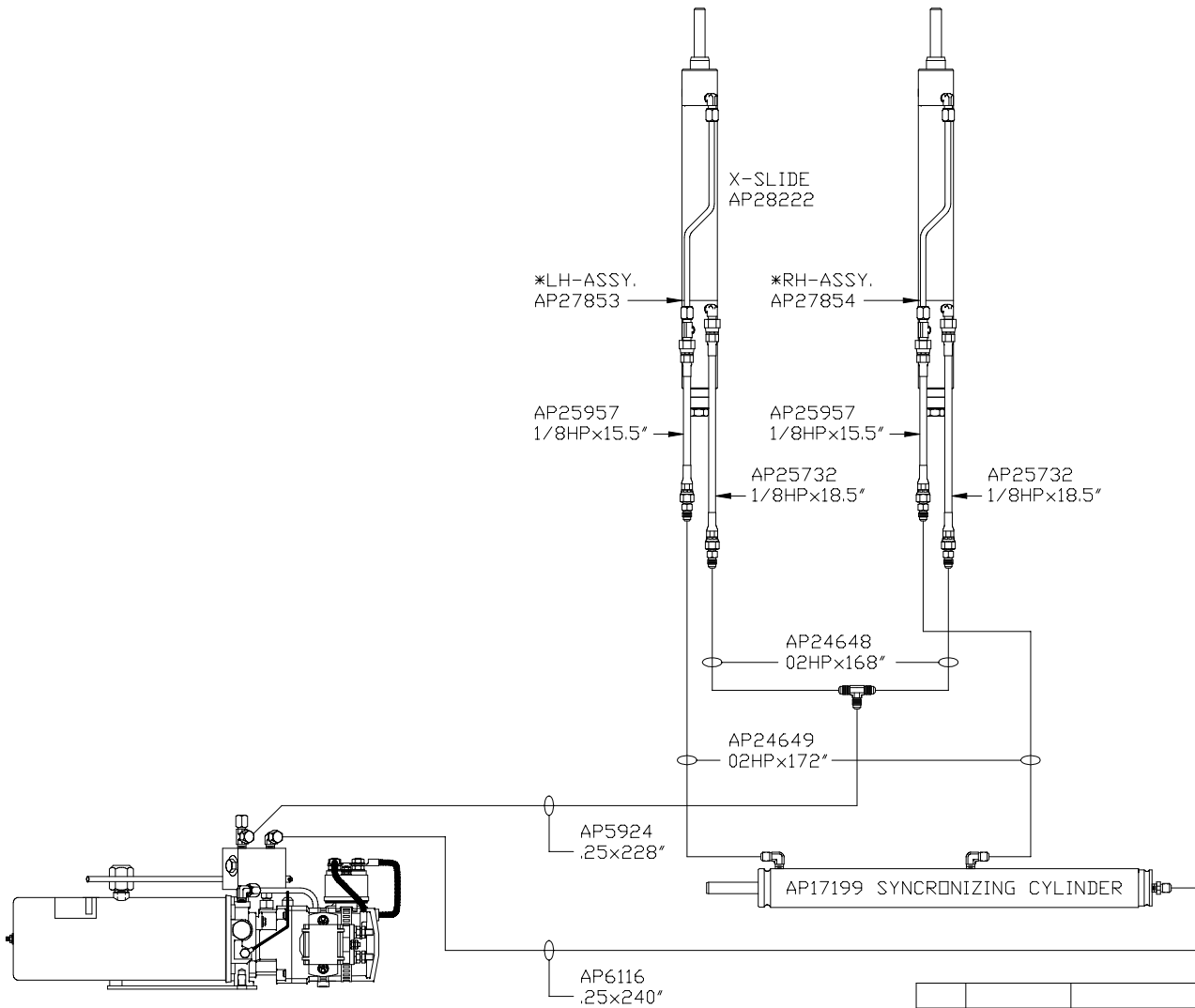
SIDE VIEW POWER UNIT-AP28608
