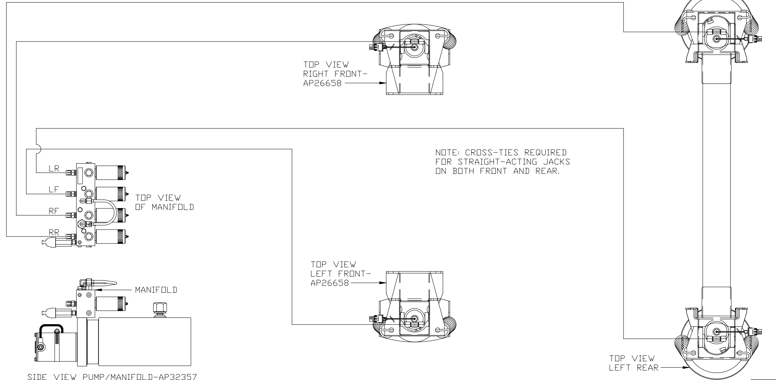
SIDE VIEW PUMP/MANIFOLD-AP32357
