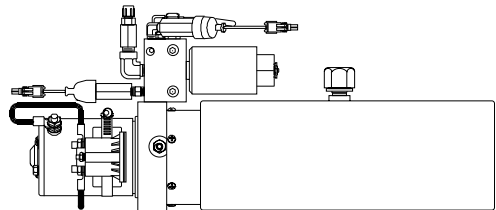
SIDE VIEW PUMP/MANIFOLD-AP38486
