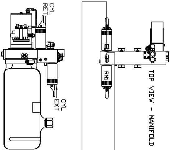
SIDE VIEW PUMP/MANIFOLD-AP44522 LOCATION AND ORIENTATION OF PUMP/MANIFOLD ASSEMBLY WILL DIFFER DEPENDING UPON O.E.M.
