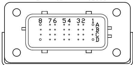
FRONT VIEW - AP52365
