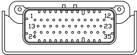
FRONT VIEW - AP58701-02
